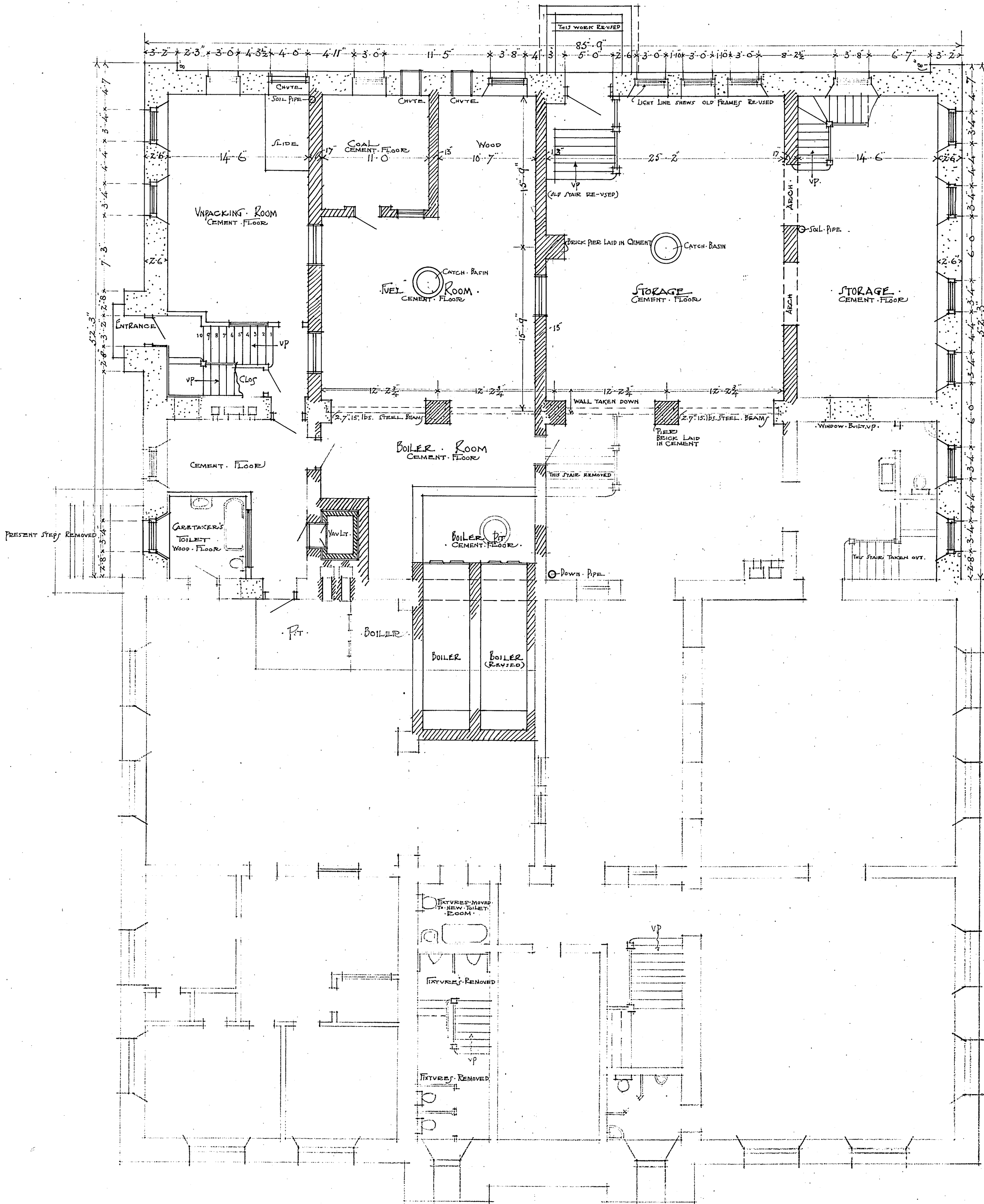
BASEMENT PLAN
